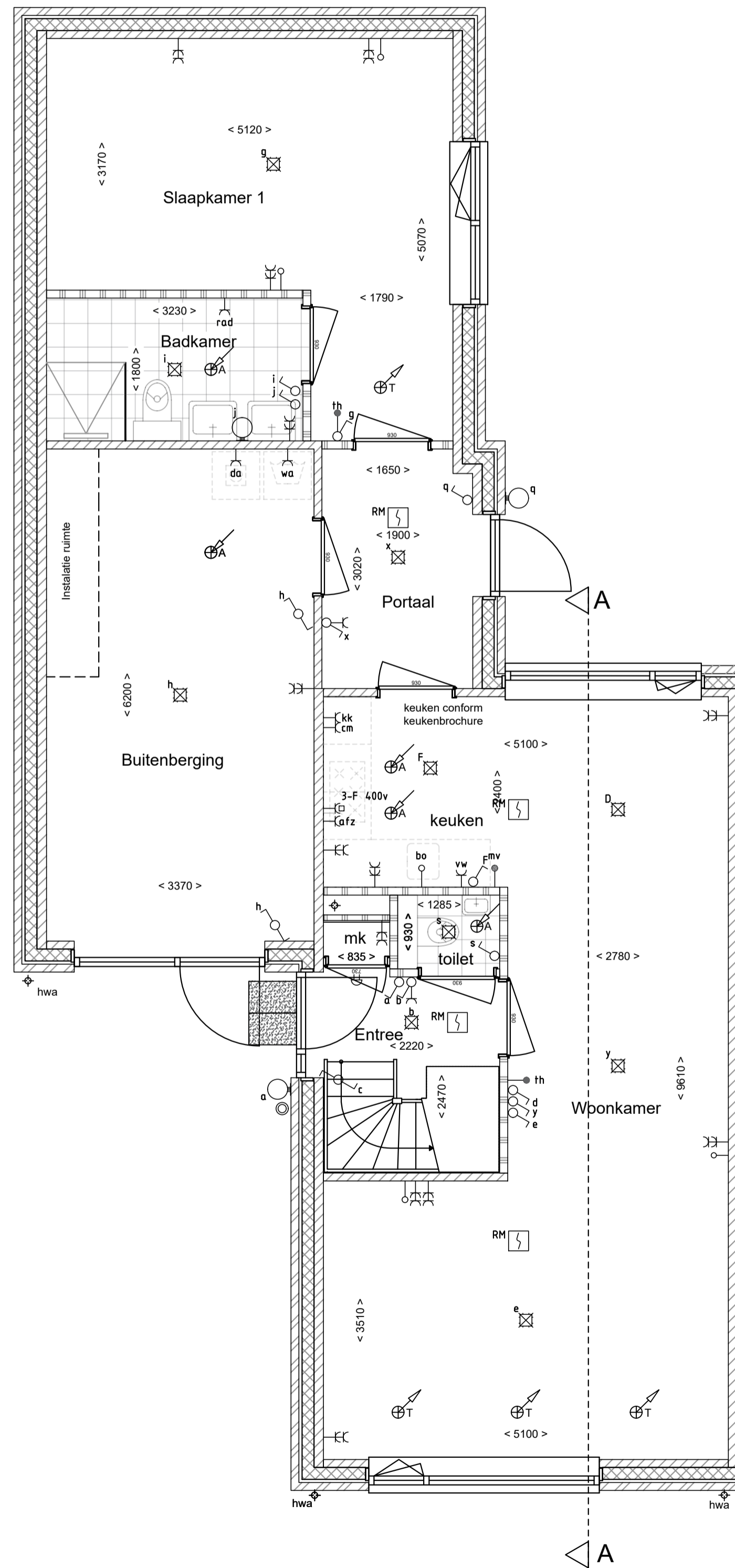
Beganegrand
